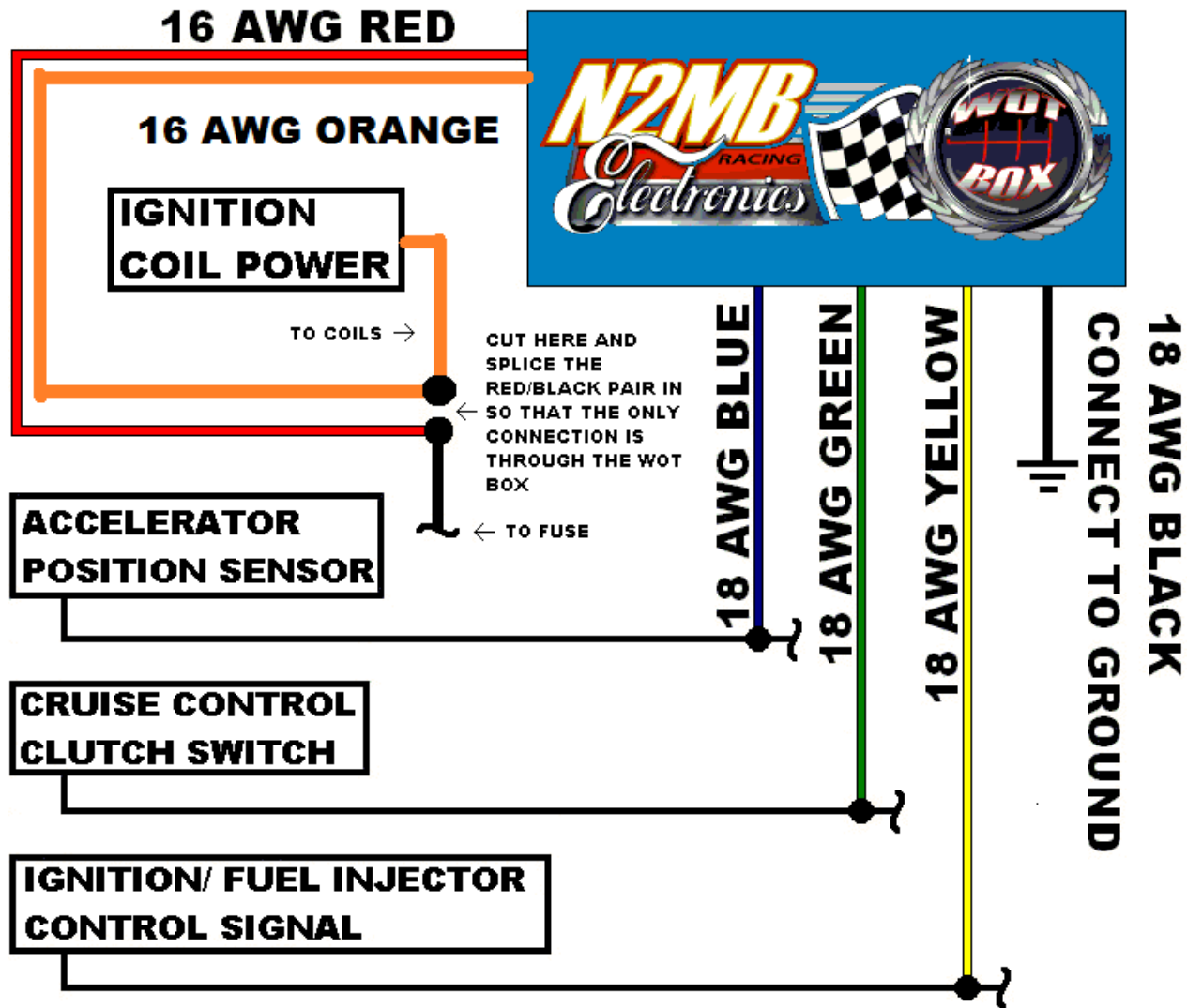
Figure I: Installation schematic
